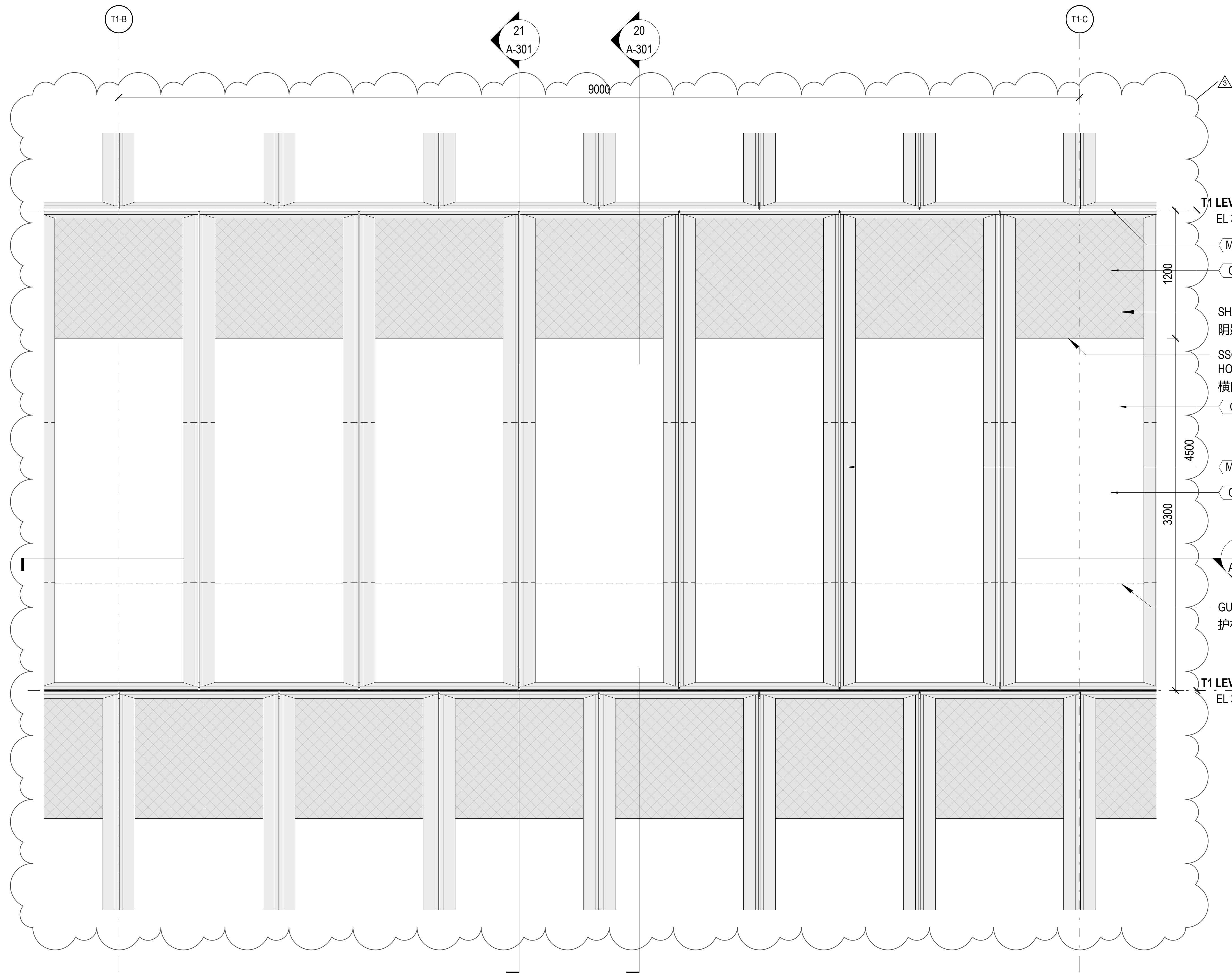
23 TOWER CW (CW-1)- ELEVATION T1号楼典型幕墙(CW-1)-立面 1 : 20
