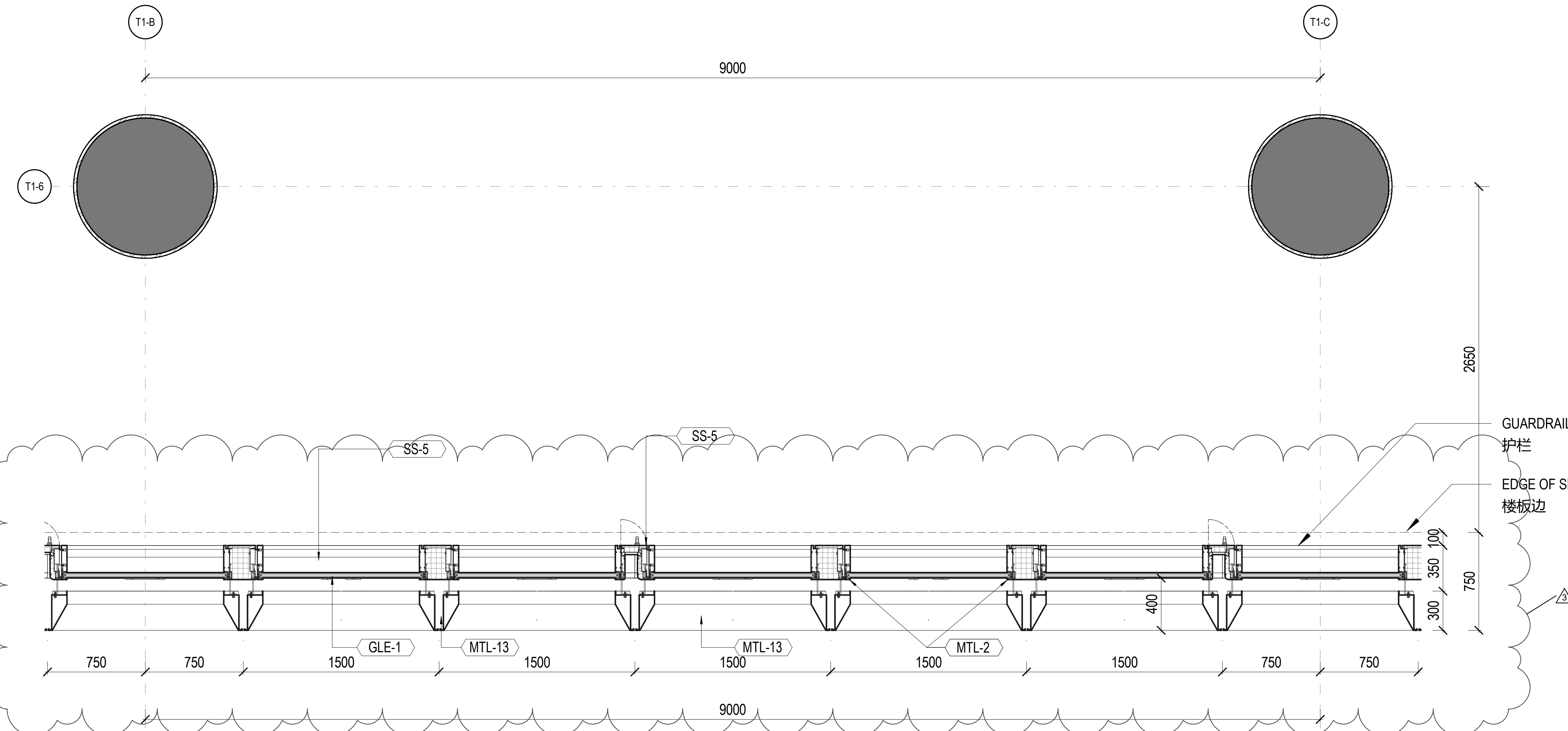
11 TOWER CW (CW-1) - PLAN T1号楼典型幕墙(CW-1)-平面 1 : 20
