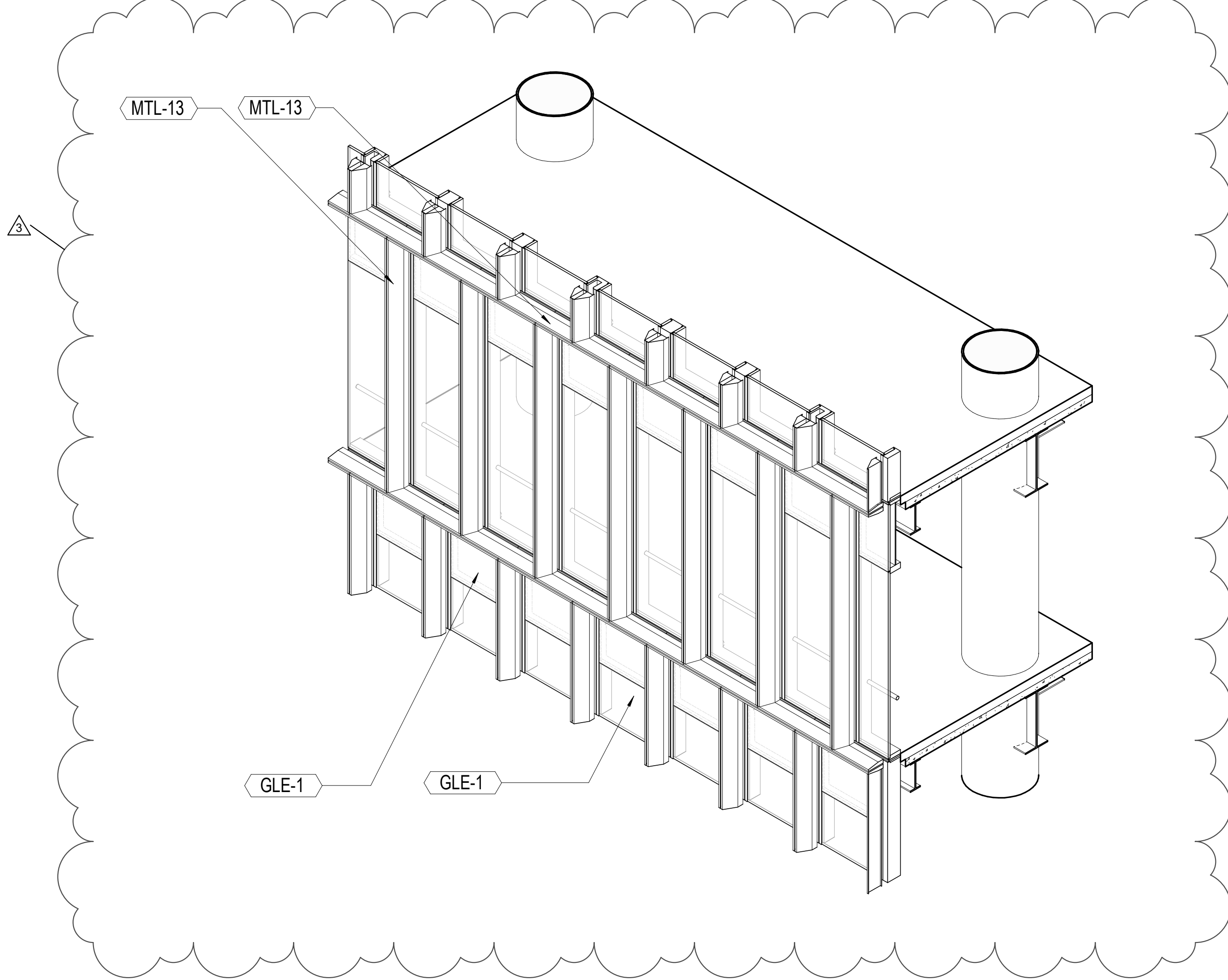
10 TOWER CW-1 TYPICAL - AXON T1号楼塔楼典型幕墙(CW-1)-轴测图
